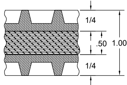
SECTION A-A (STANDARD CAPACITY SHOWN)
